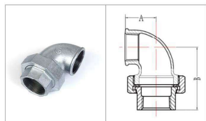
Fig.97 Union Elbow Flat Seat MF
