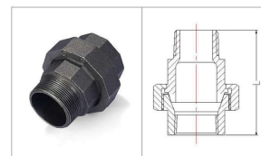
Fig.341 Union, Taper Seat, M&F
