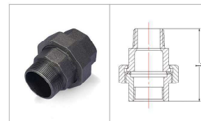
Fig.340 Union, Taper Seat
