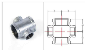
Fig.180R Crosses, Reducing
