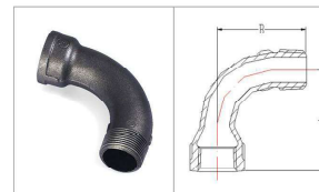
Fig.1 90 Degree M&F Long Sweep Bends
