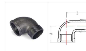
Fig.92 90° M&F Elbow, Equal
