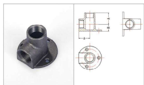
Fig.529 Socket M&F
