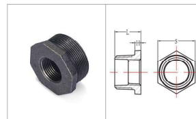
Fig.241 Bushings
