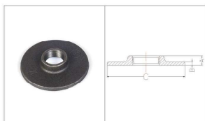
Fig.321 Round Flange, Without Bolt Hole
