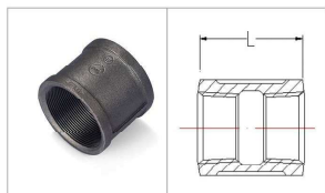
Fig.220 Part Thread Sockets
