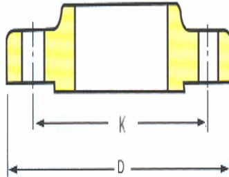
SLIP-ON RF
